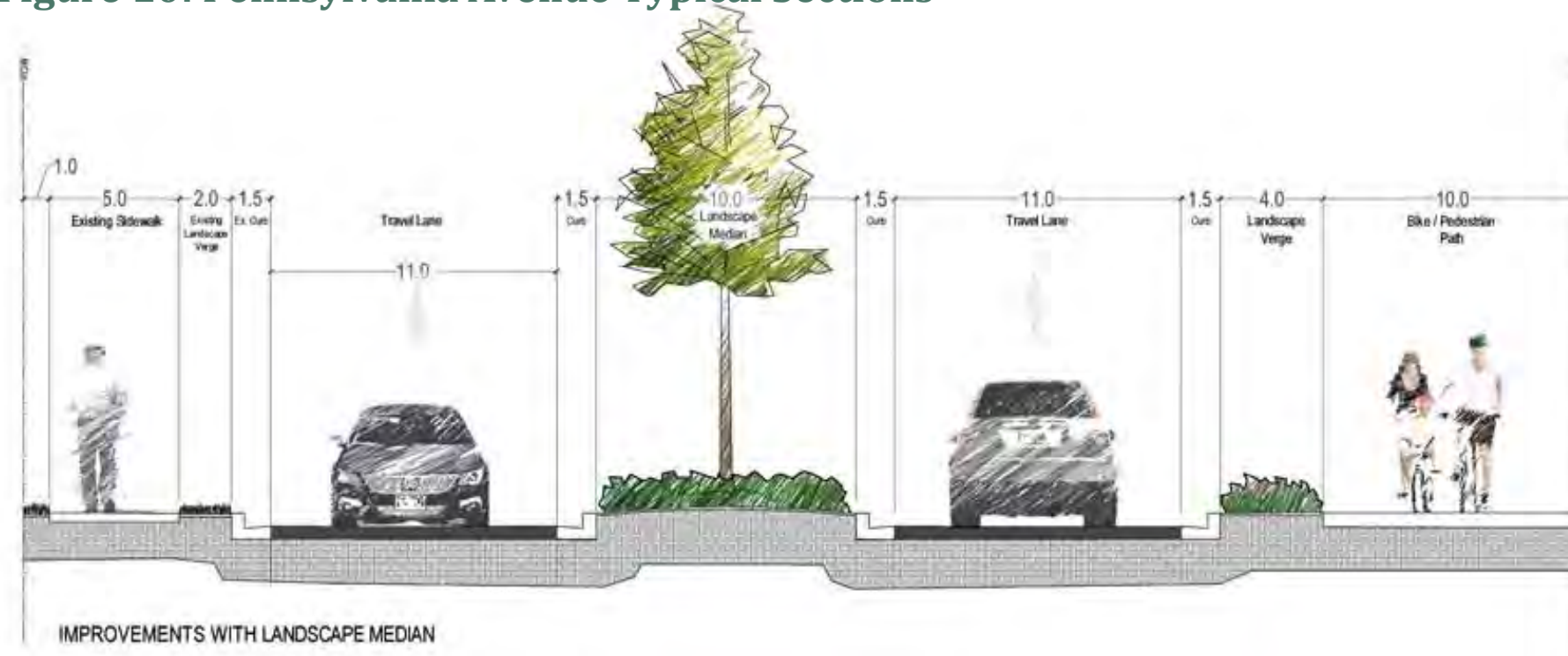
Figure 10: Pennsylvania Avenue Typical Sections
