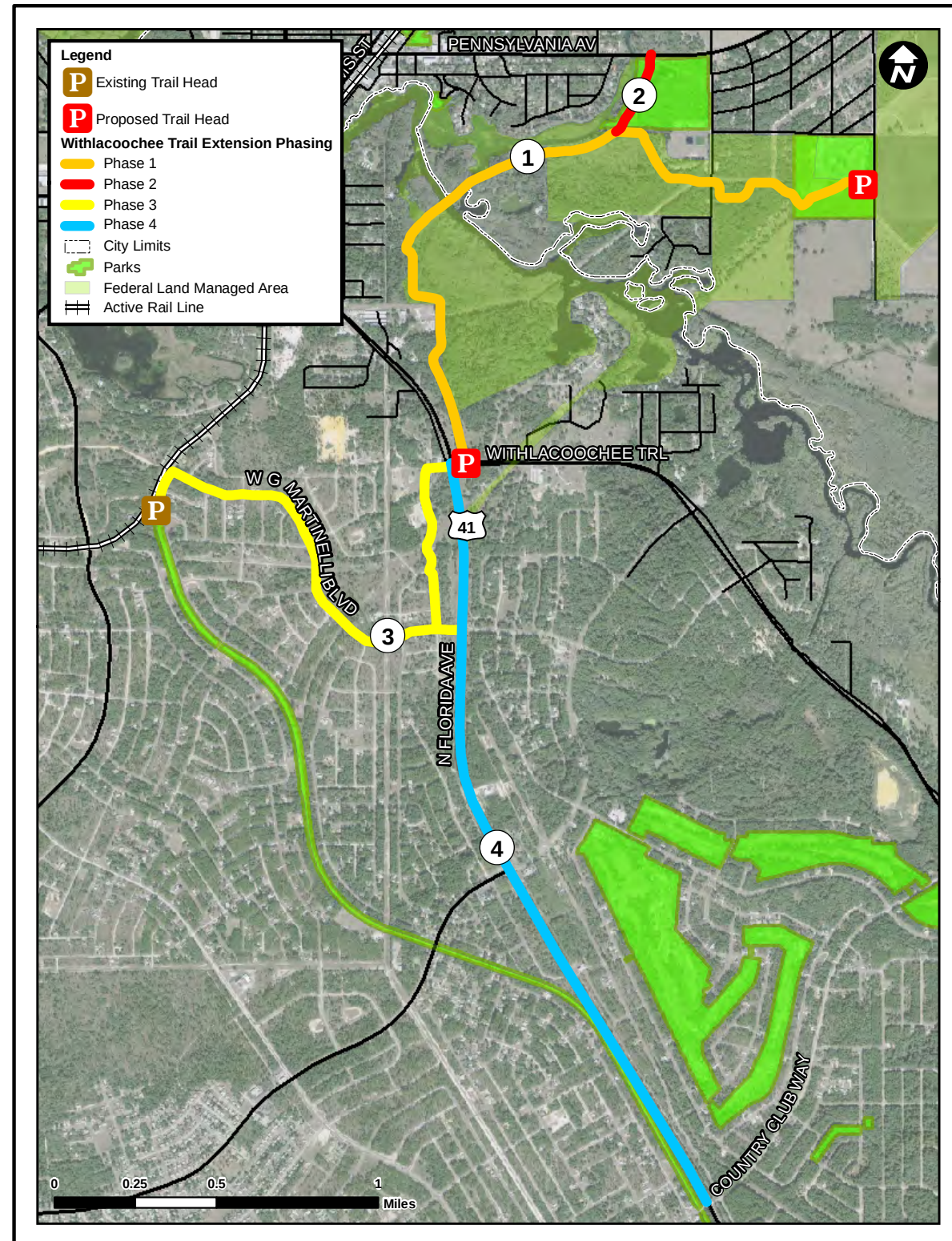
Figure 7: Withlacoochee Trail Extension Phases
