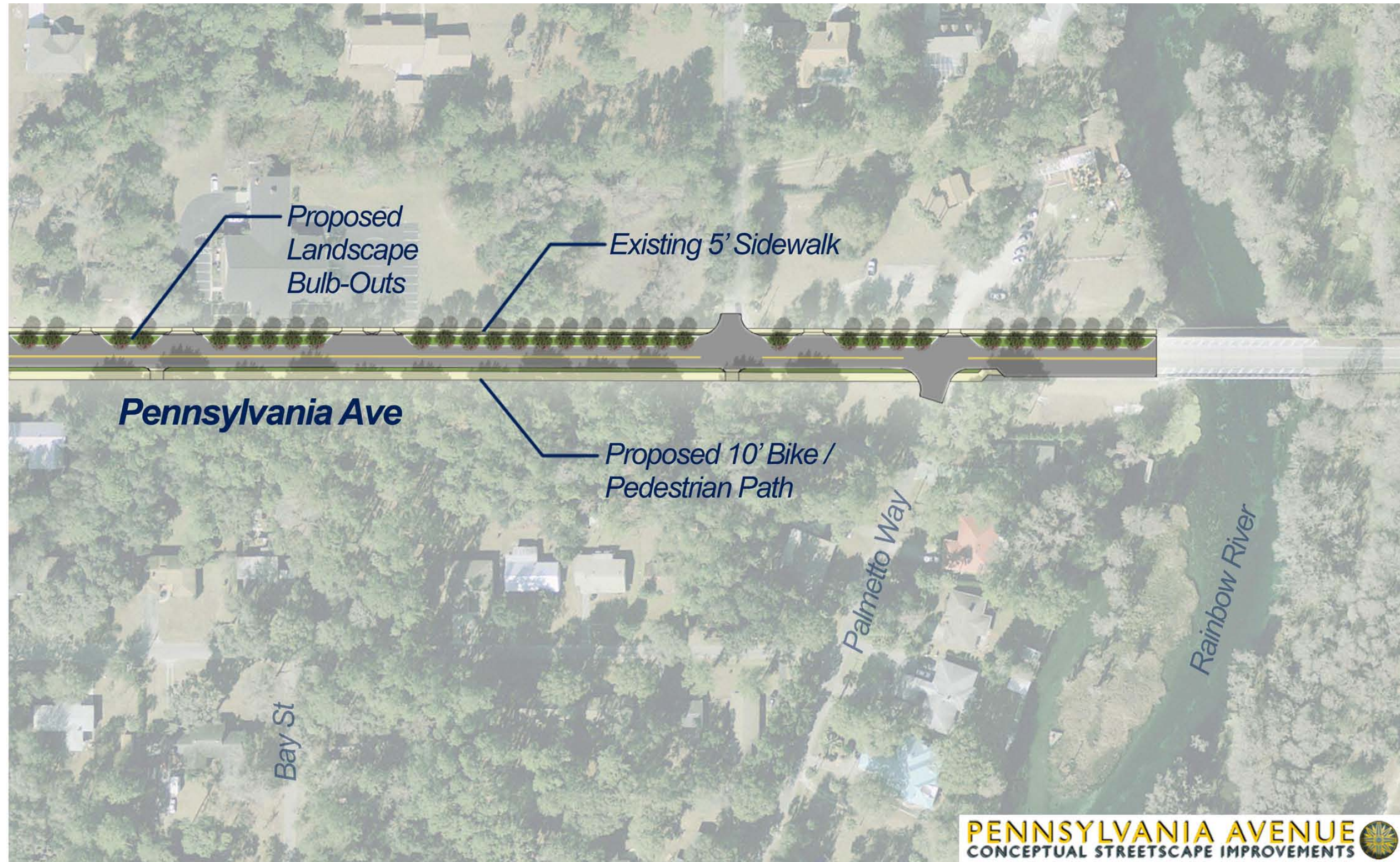
Figure 9D: Pennsylvania Avenue Streetscape Plan View - East
