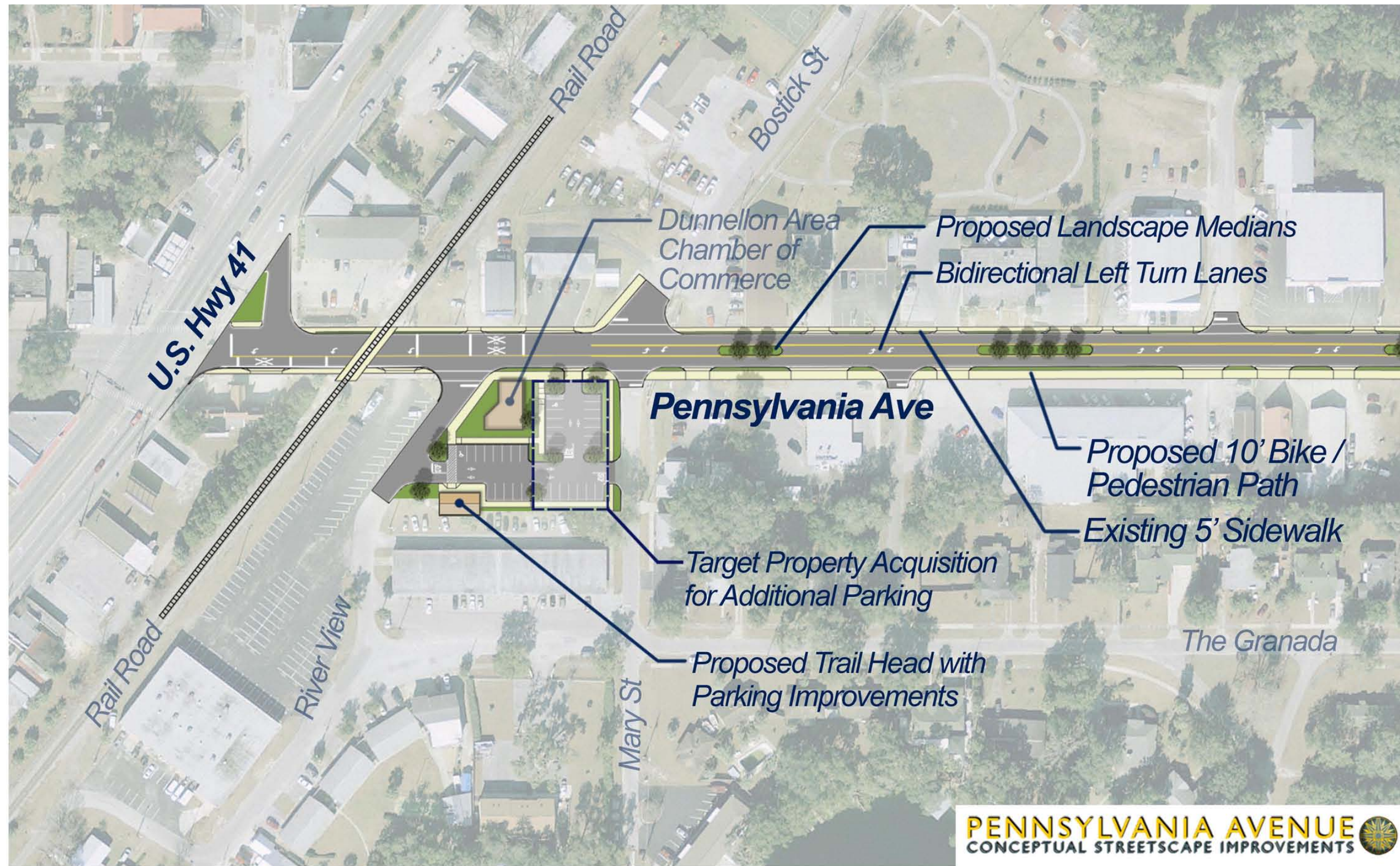
Figure 9B: Pennsylvania Avenue Streetscape Plan View - West
