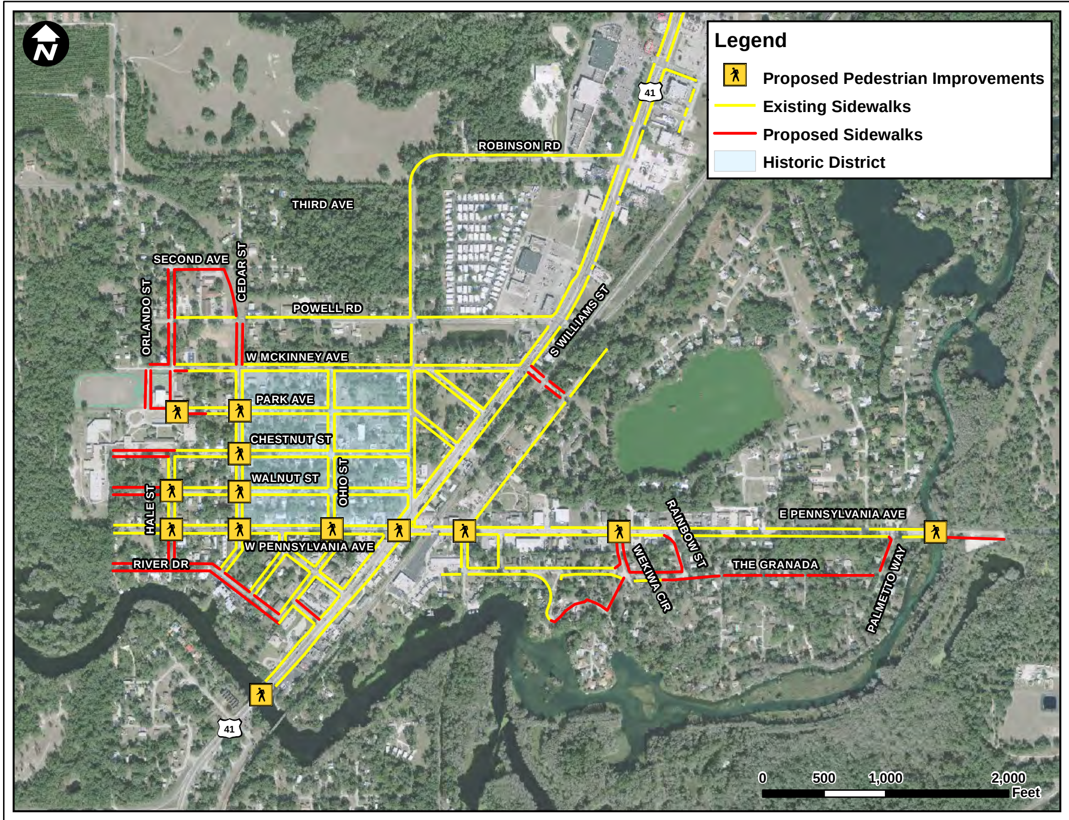
Figure 14: Pedestrian Facility Improvements
