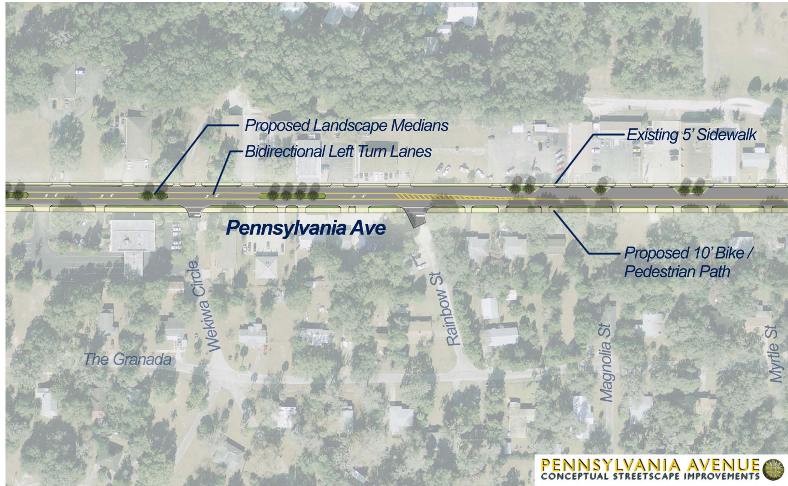
Figure 9C: Pennsylvania Avenue Streetscape Plan View - Center
